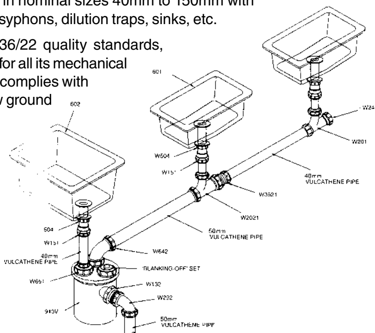
Vulcathene Mechanical Jointing System
