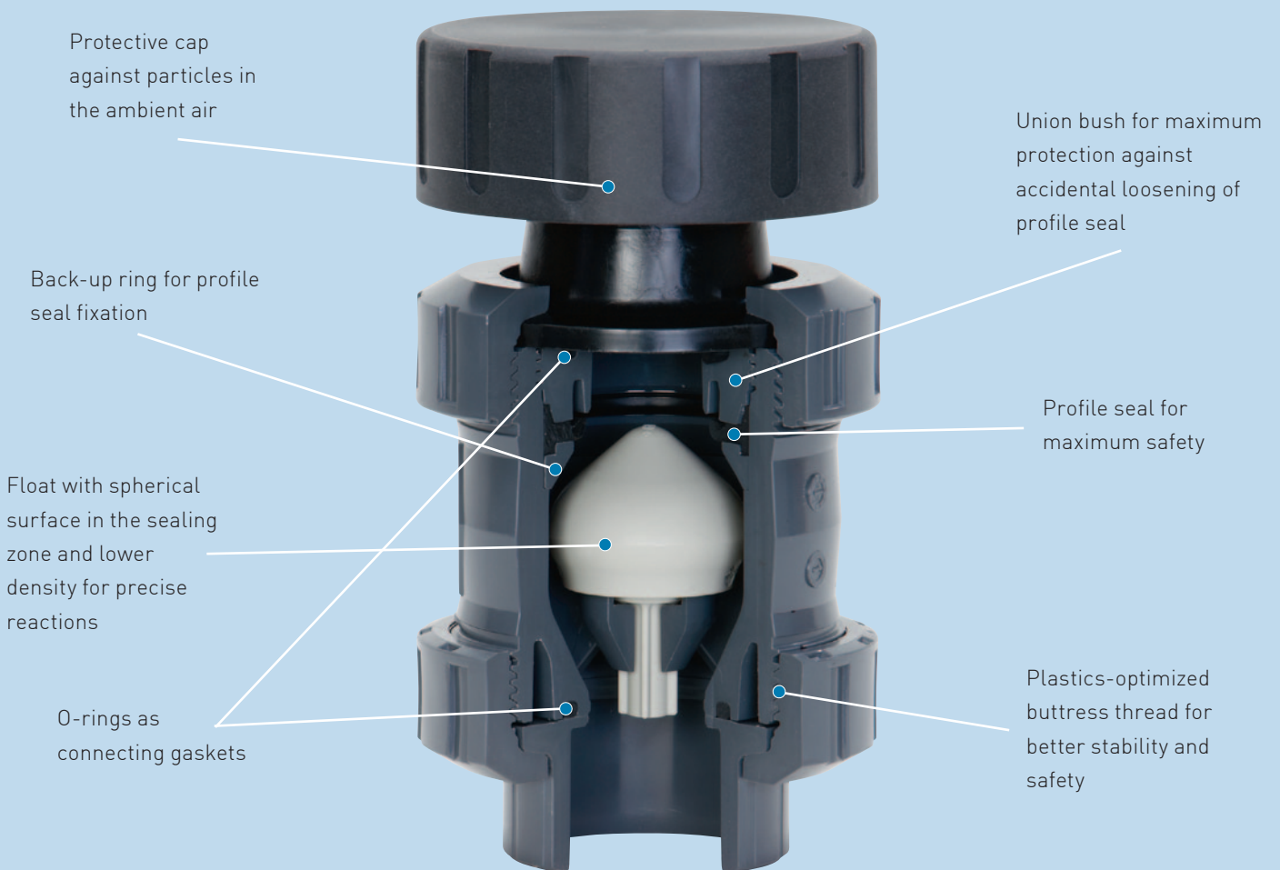
Ventilating- and Bleed valve type 591: without spring (illustration above) Ventilating valve type 595: with spring
